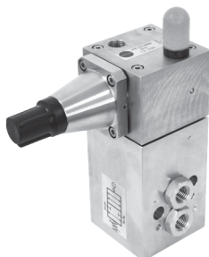
Fig. 36: Type 3709-5 Pneumatic Lock-up Valve
